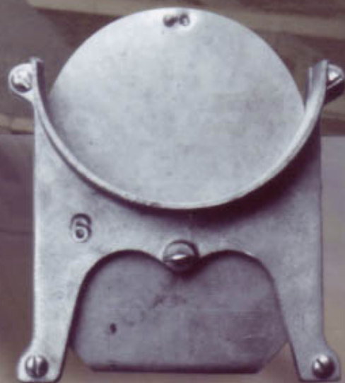
Aluminum Half Blast Gate Cut-Offs
